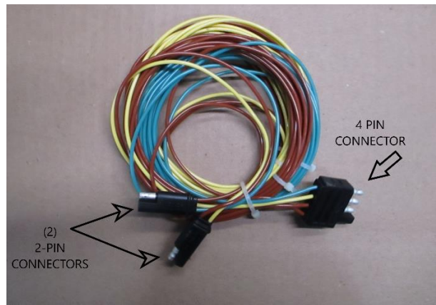
Rear Wiring Harness ( Part C )
