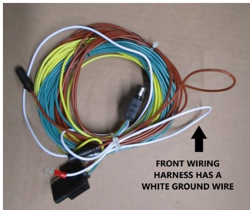
Front Wiring Harness ( Part B )
